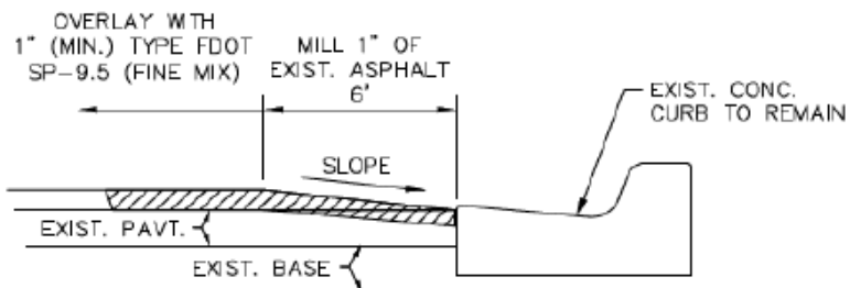
ASPHALT TRANSITION DETAIL ADJACENT TO CURB
