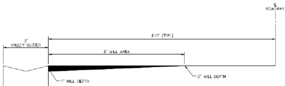
MILLING CROSS-SECTION DETAIL NOT TO SCALE
